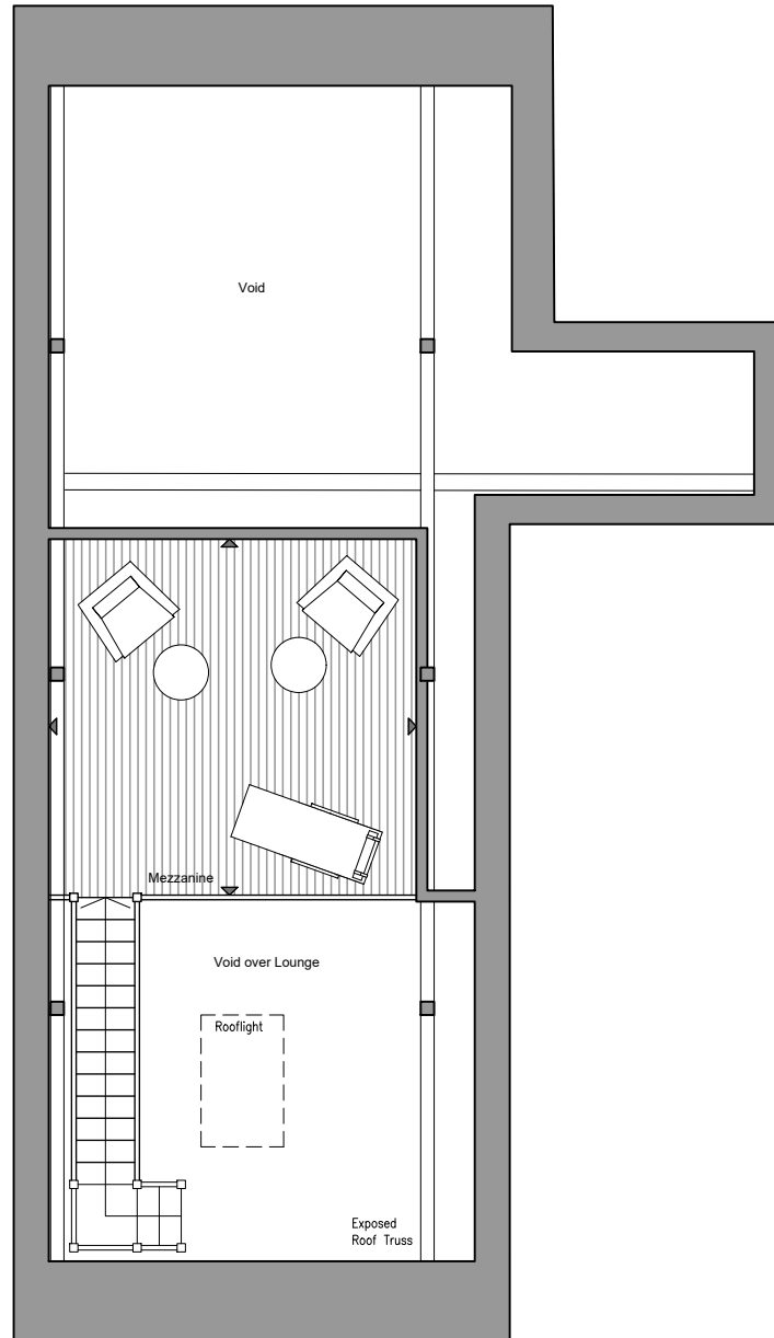
Mezzanine Floor
